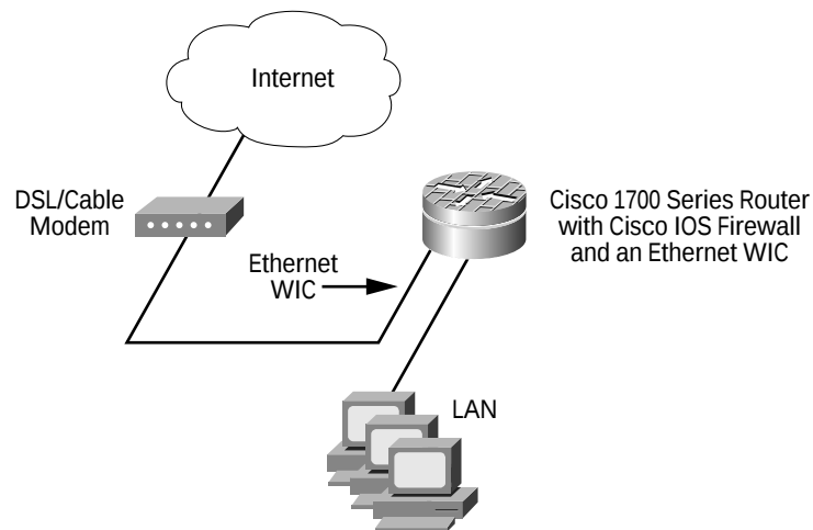
Figure 3: The Cisco 1700 Series Deployed with an Ethernet WIC and an External DSL or Cable Modem
