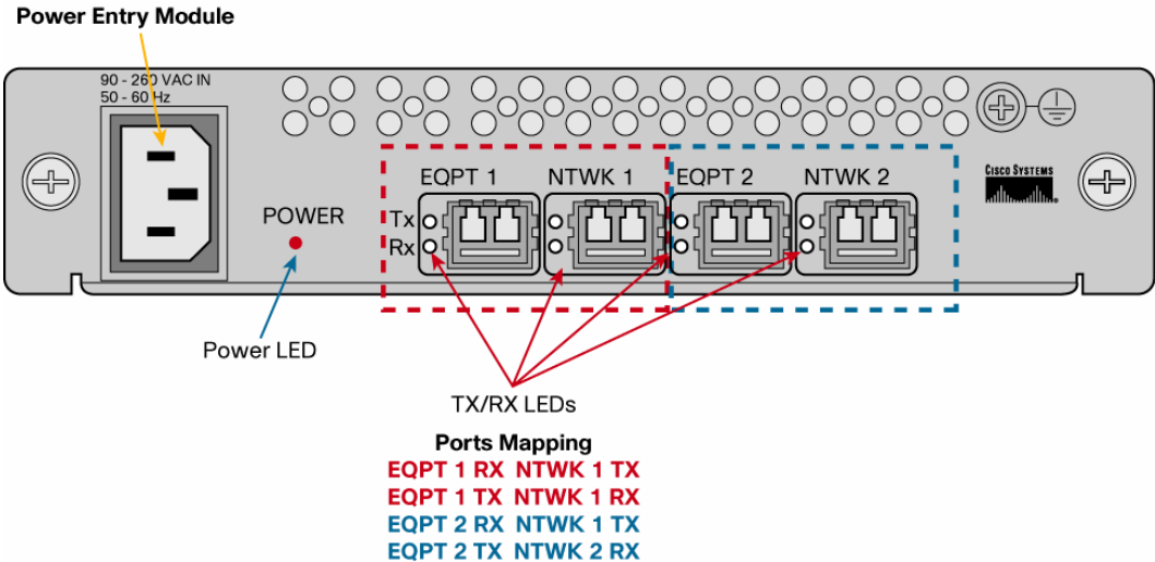
Figure 5. Front-Panel LEDs
