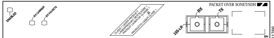
Figure 1-2 PA-POS-OC3SML—Faceplate View, Horizontal Orientation
