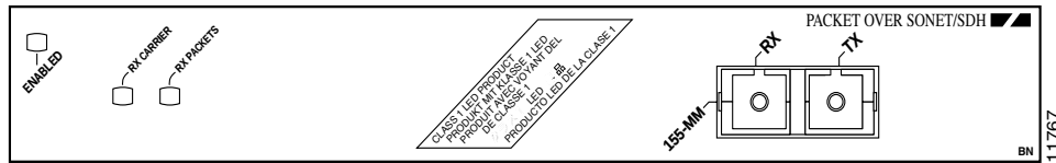
Figure 1-1 PA-POS OC3MM—Faceplate View, Horizontal Orientation
