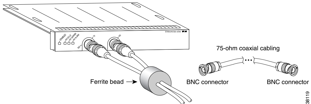
Figure 1-9 PA-A6-T3 and PA-A6-E3 Cables
