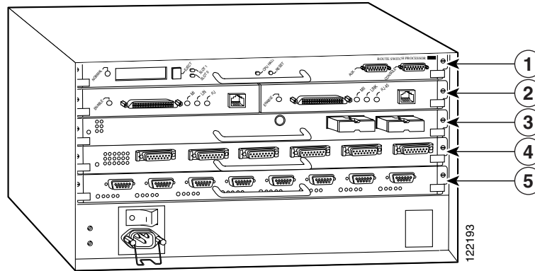
Figure 1-18 VIP Slots in the Cisco 7505 Router
