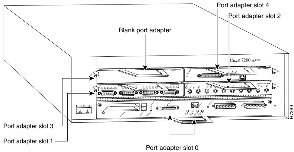
Figure 1-11 Port Adapter Slots in the Cisco 7204VXR Router
