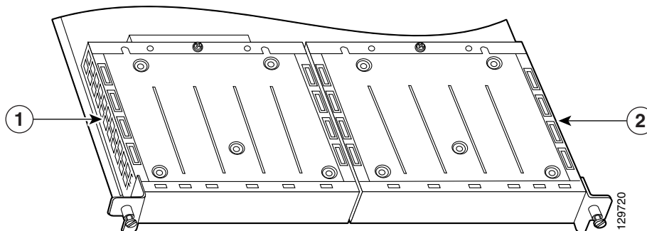
Figure 1-17 VIP Slot Locations
