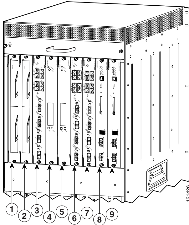
Figure 1-23 FlexWAN and Enhanced FlexWAN Slots in the Cisco 7609 Router
