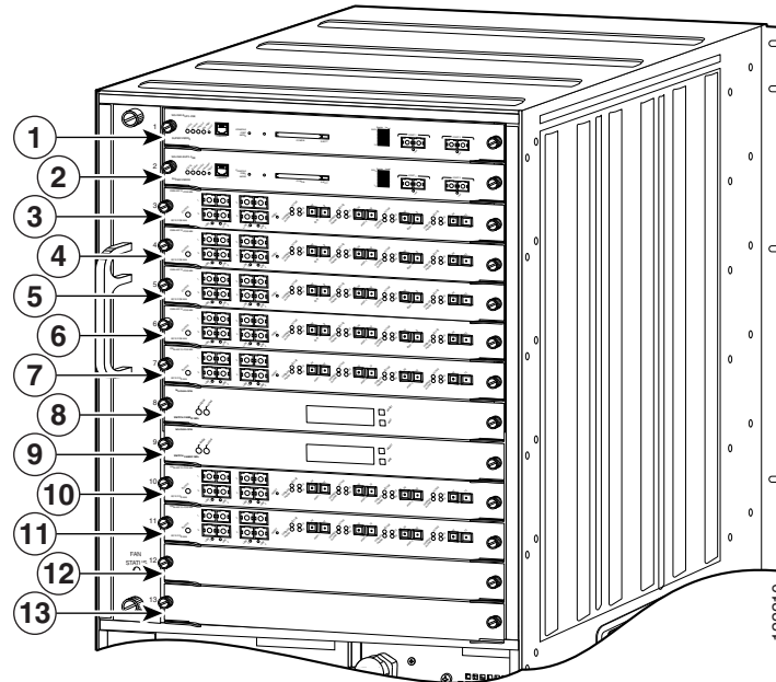
Figure 1-24 FlexWAN and Enhanced FlexWAN Slots in the Cisco 7613 Router
