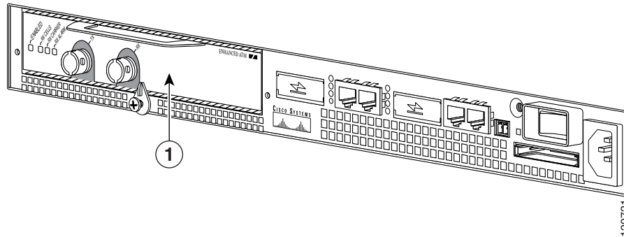
Figure 1-16 Port Adapter Slot in the Cisco 7401ASR Router
