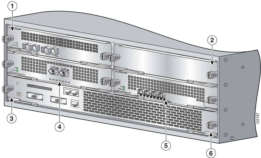
Figure 1-15 Module Slots on the Cisco 7304 Router
