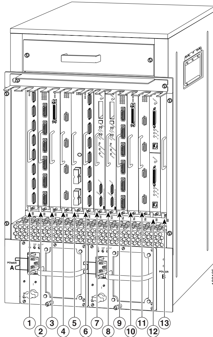
Figure 1-20 VIP Slots in the Cisco 7513 Router
