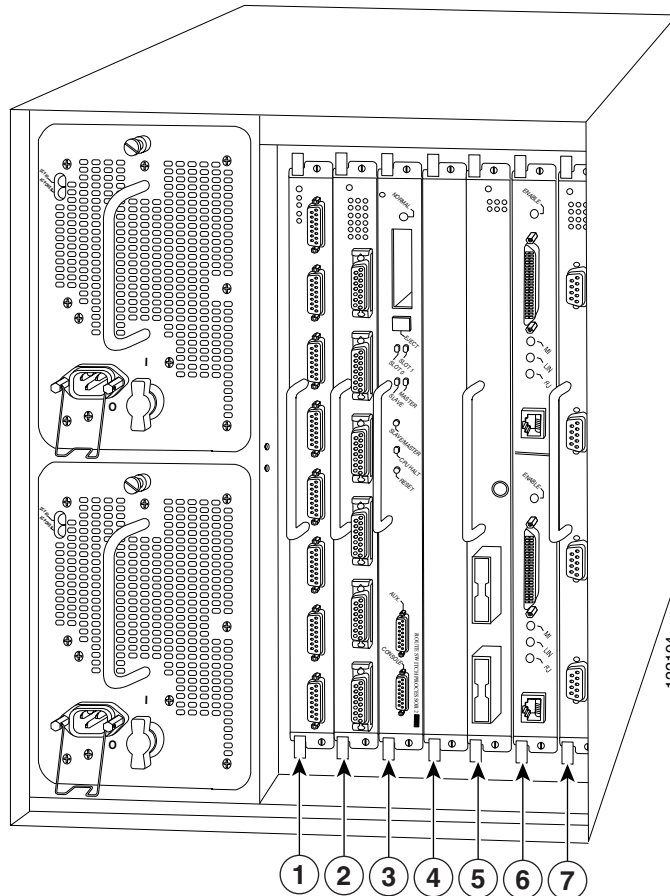
Figure 1-19 VIP Slots in the Cisco 7507 Router
