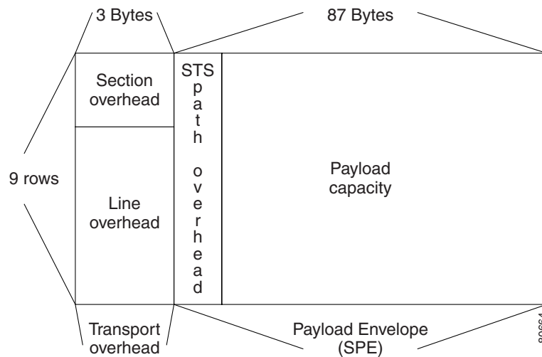
Figure 1-10 Three SONET Layers of a SONET Frame
