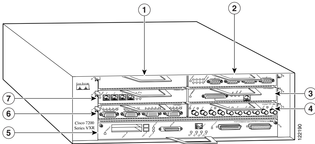
Figure 1-12 Port Adapter Slots in the Cisco 7206VXR Router
