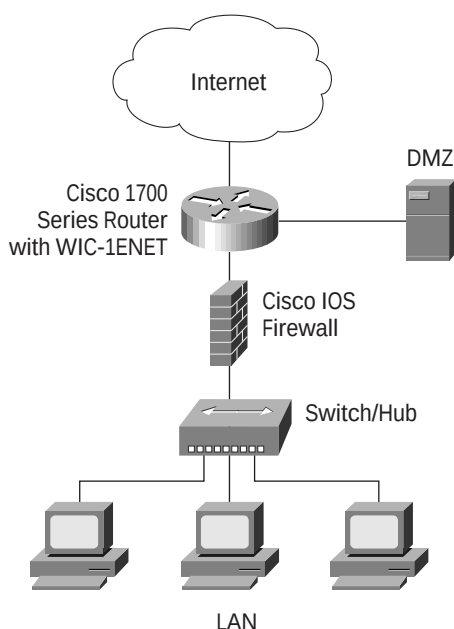
Figure 3 Configuring a Cisco 1700 Series Router for a Perimeter LAN or DMZ
