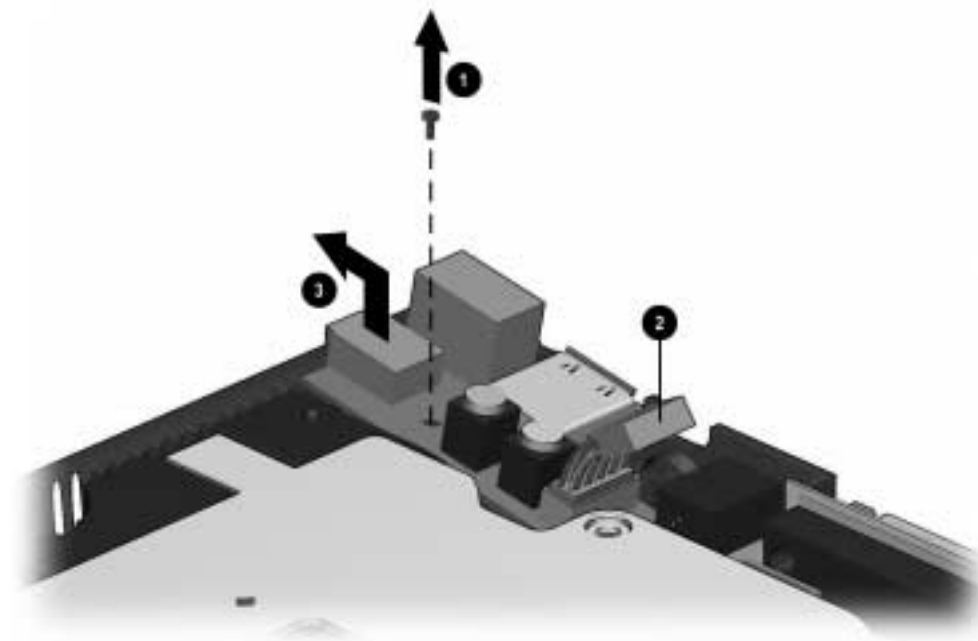
Figure 5-31. Removing the USB Board
