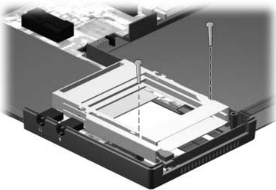
Figure 5-36. Removing the PC Card Assembly Screws
