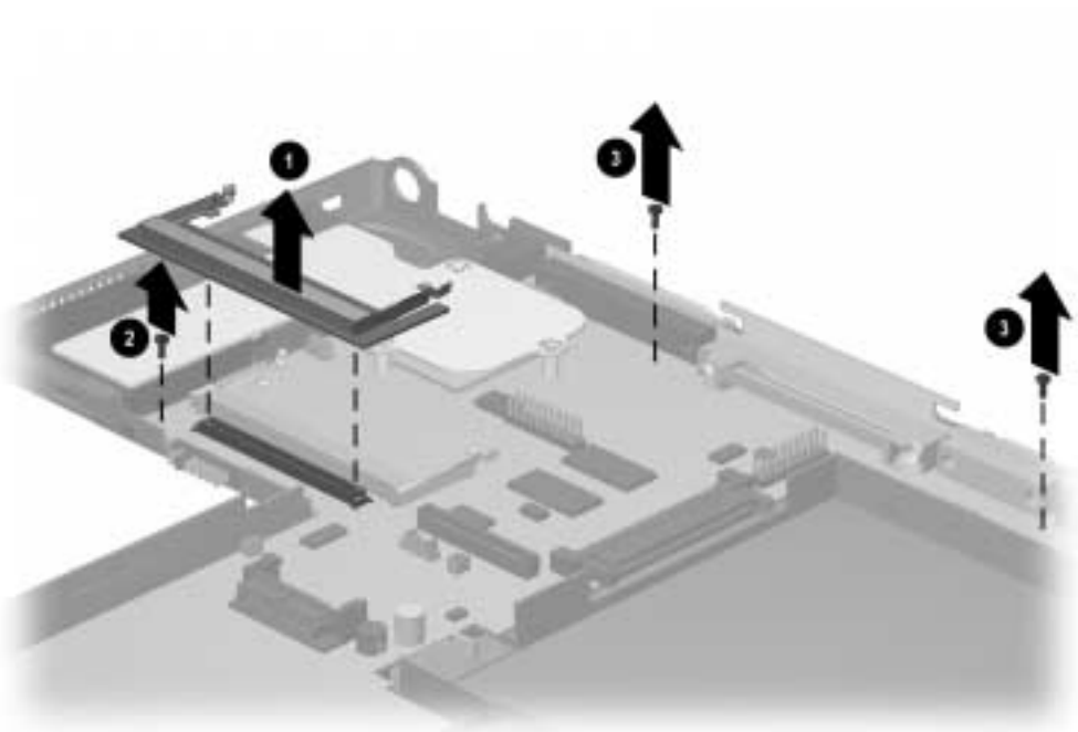
Figure 5-35. Removing the Memory Bracket/Connector and System Board Screw
