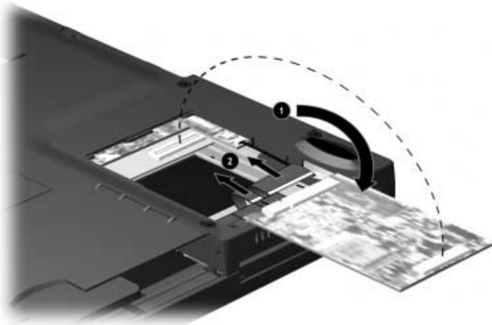
Figure 5-16. Removing a Modem/Combo Card
