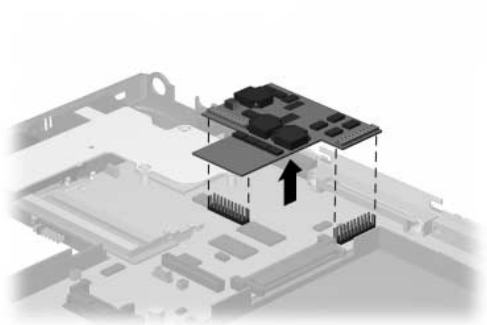
Figure 5-32. Removing the Voltage Converter Board
