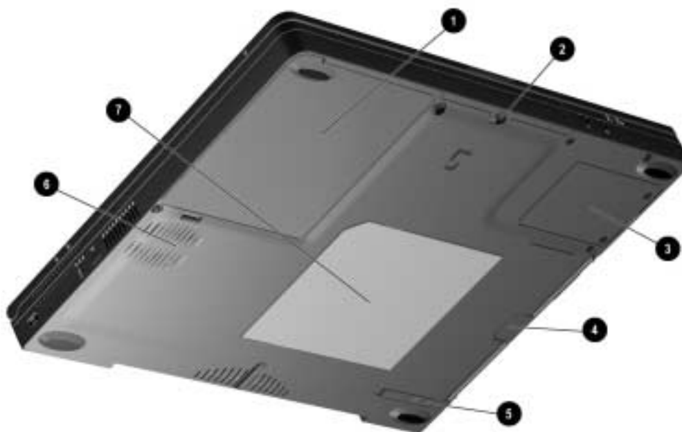
Figure 1-7 Bottom Components
