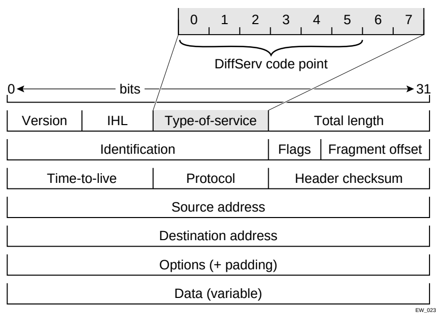
Figure 25: IP packet header encapsulation
