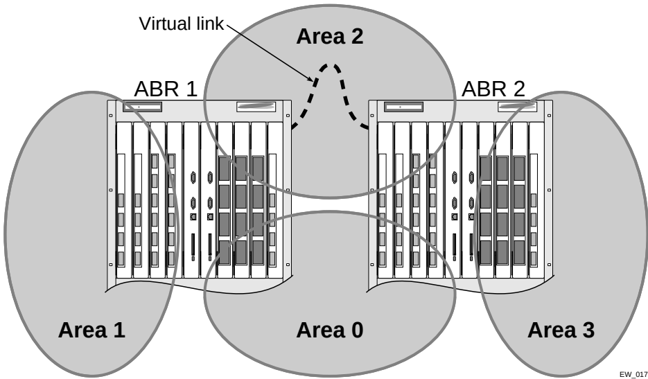
Figure 31: Virtual link providing redundancy
