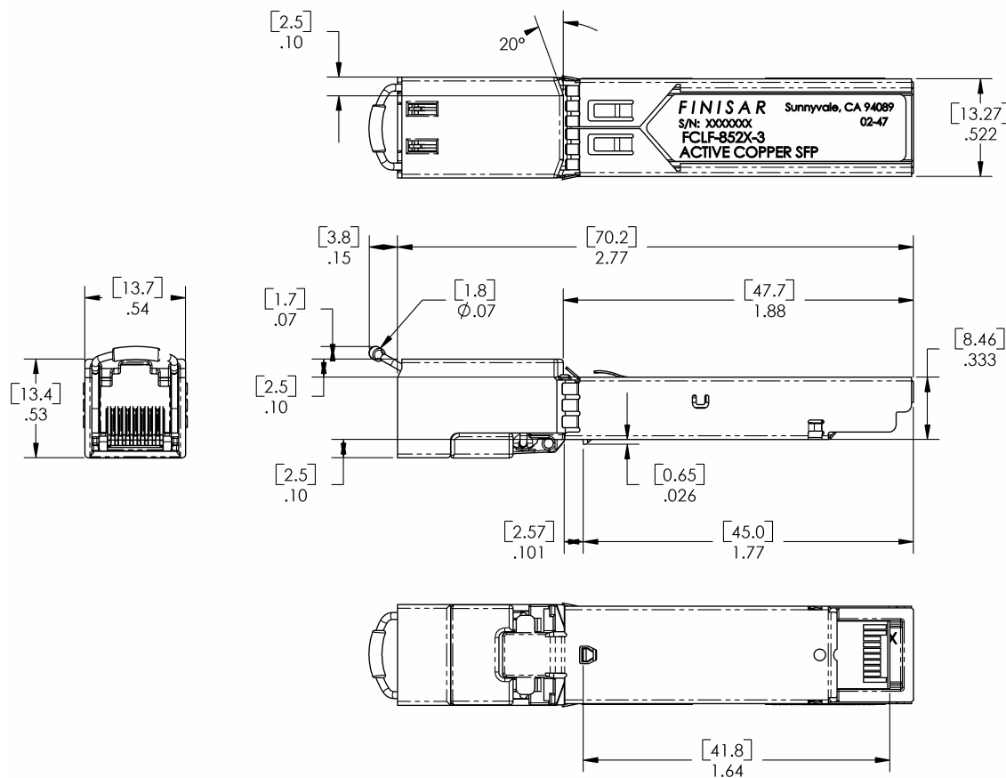
Figure 2. FCLF-8520/8521-3 mechanical dimensions
