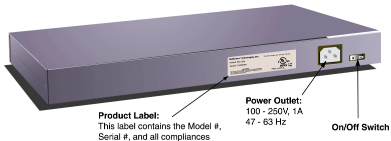
Figure 1-3 Back Panel of the NetScreen-10
