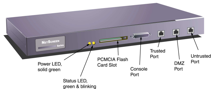
Figure 1-1 Front Panel of the NetScreen-10
