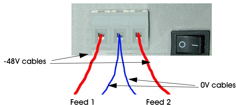
Figure: DC Power Supply Cabling
