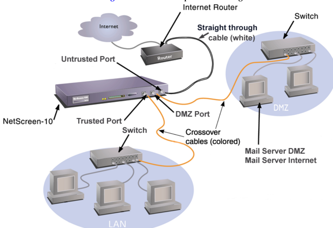
Figure 2-5 Sample Configuration Using DMZ Port
