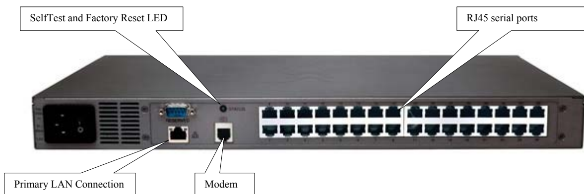
Figure 2 Rear Panel
