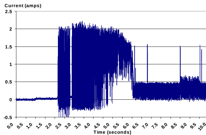
Figure 1. Typical startup and operation current profile
