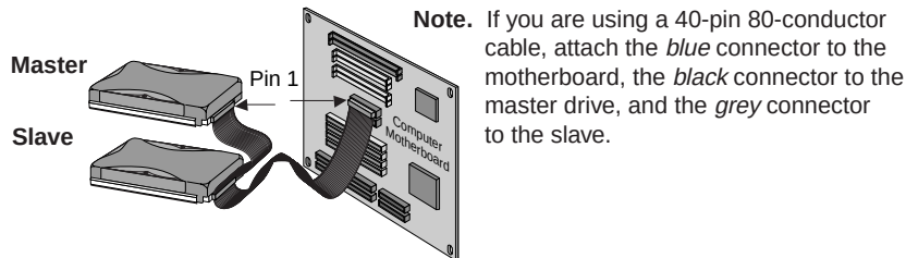
Figure 3. Ultra ATA cable connectors
