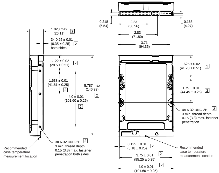
Figure 4. Mounting dimensions—top, side and end view
