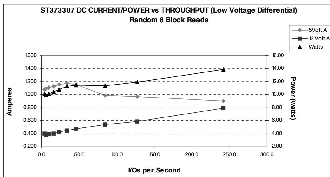
Figure 11. ST373307 DC current and power vs. input/output operations per second (LVD)
