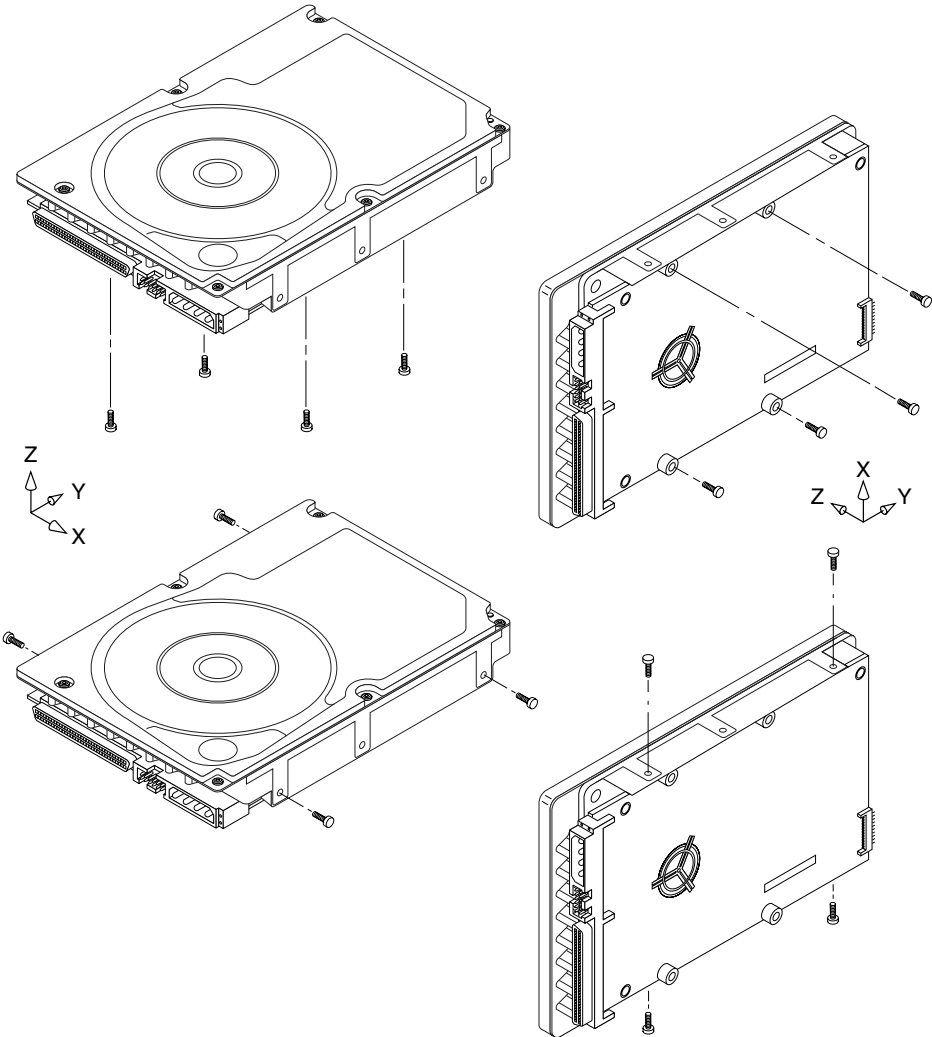
Figure 15. Recommended mounting
