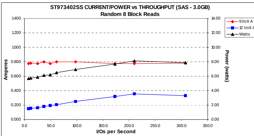
Figure 5. ST973402SS (3 Gbit) DC current and power vs. input/output operations per second
