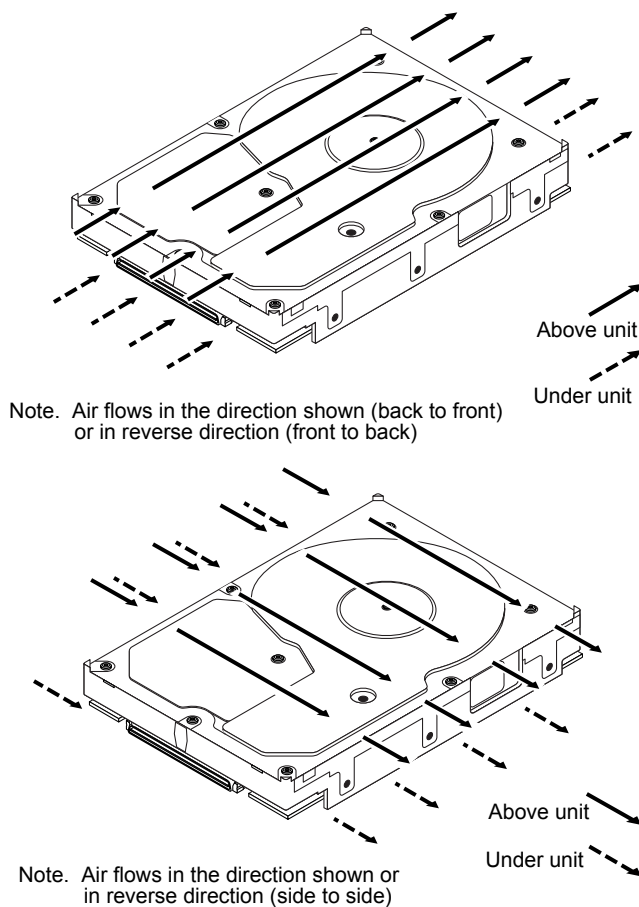
Figure 13. Air flow (suggested)
