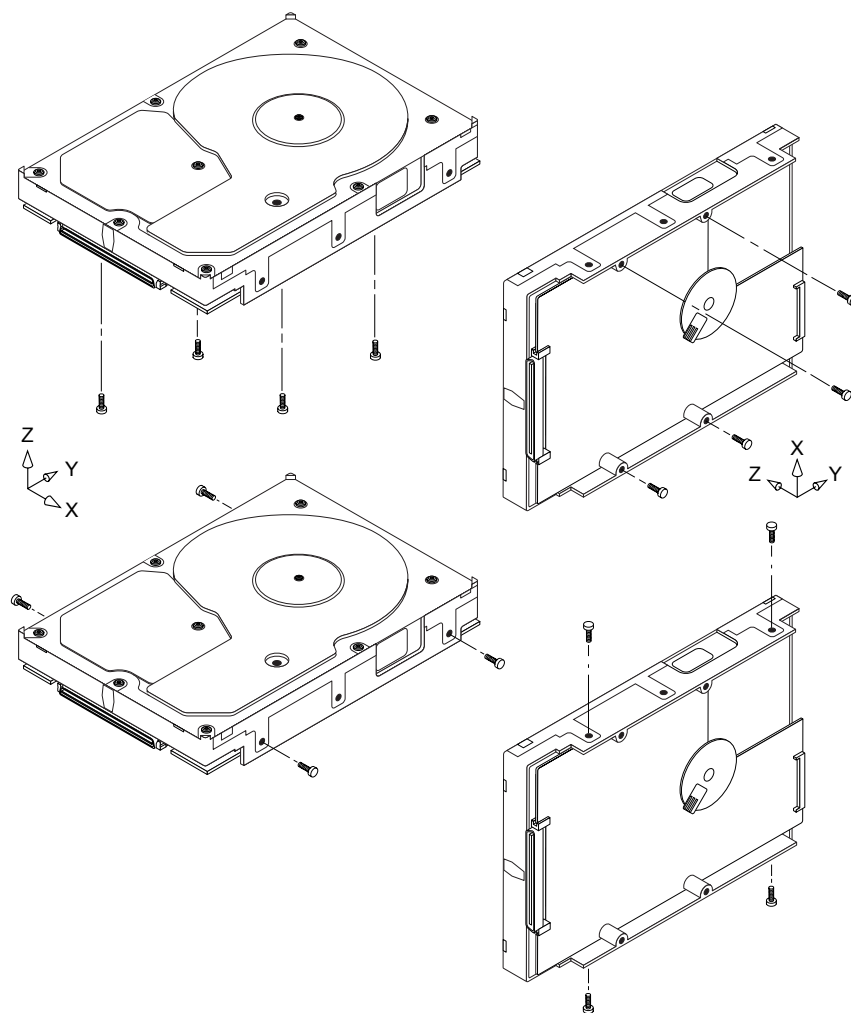
Figure 7. Recommended mounting
