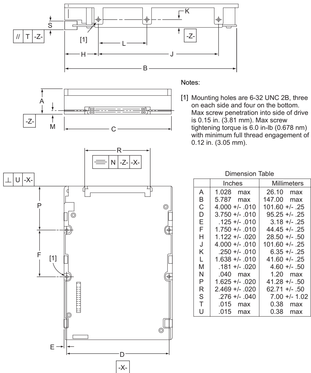
Figure 9. LC mounting configuration dimensions
