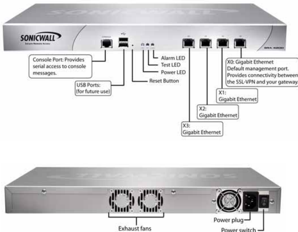
Figure 1 SonicWALL SRA 4200 Front and Back Panels
