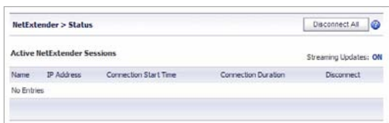
Figure 30 NetExtender > Status
