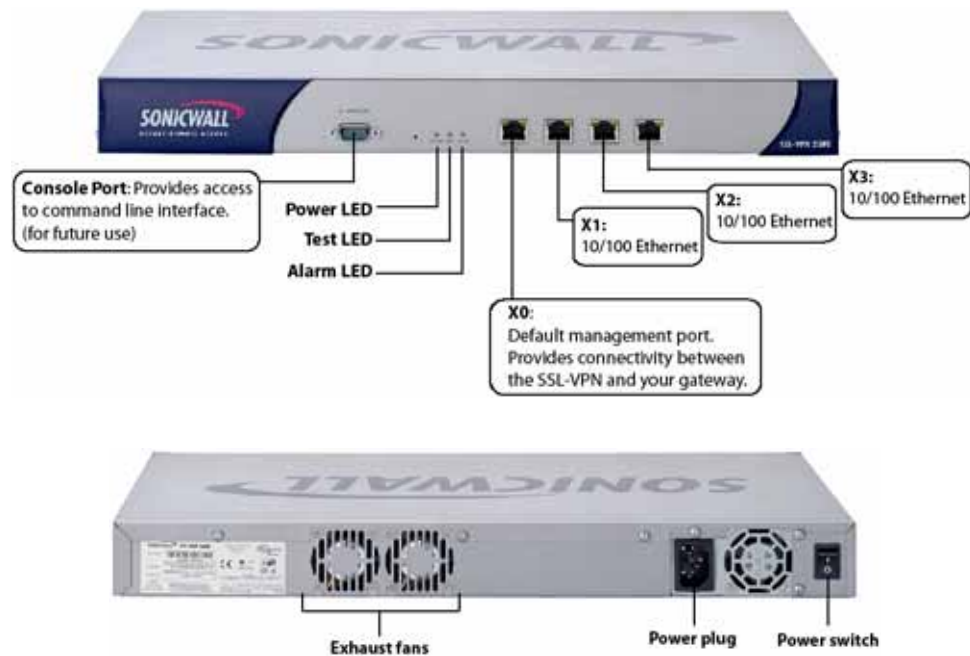
Figure 2 SonicWALL SSL-VPN 2000 Front and Back Panels
