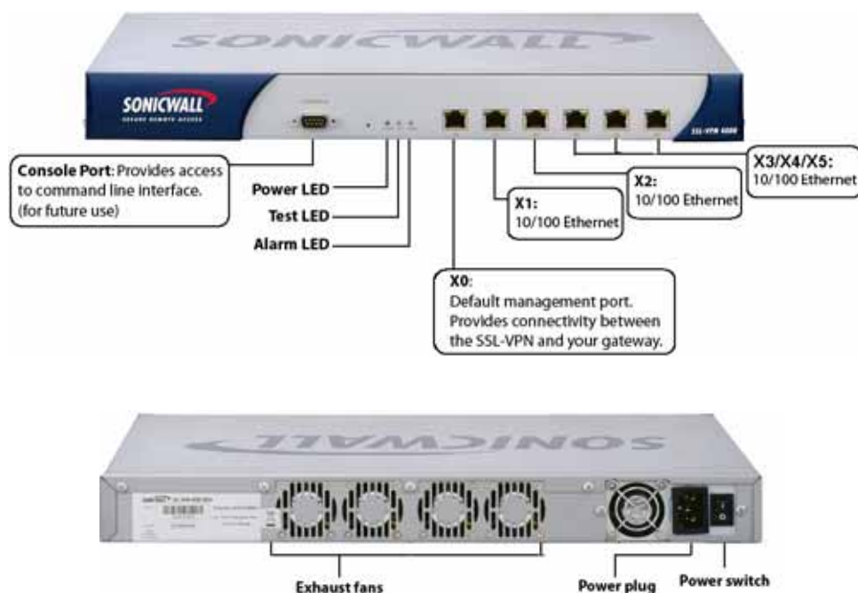
Figure 3 SonicWALL SSL-VPN 4000 Front and Back Panels
