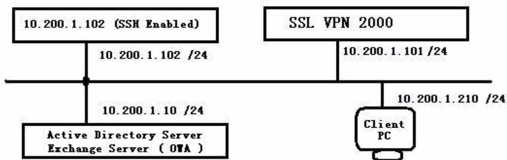
Figure 43 Network Topology
