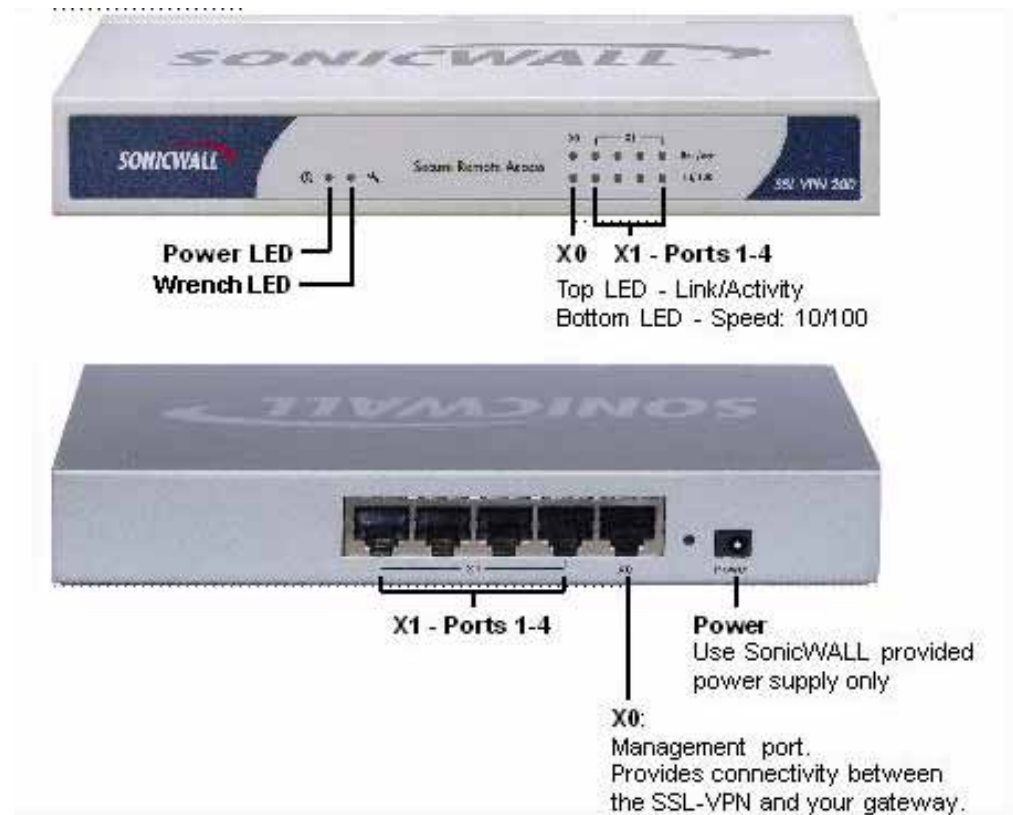
Figure 4 SonicWALL SSL-VPN 200 Front and Back Panels
