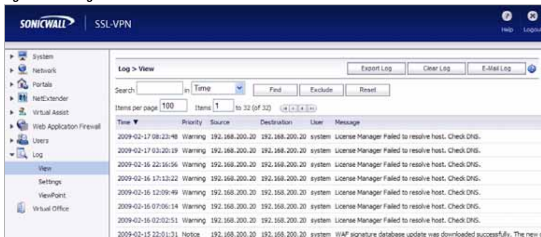
Figure 36 Log > View
