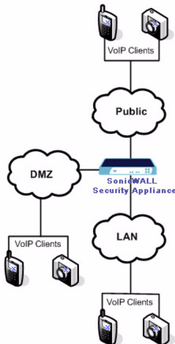
Figure 3 Point-to-Point VoIP Service Topology.
