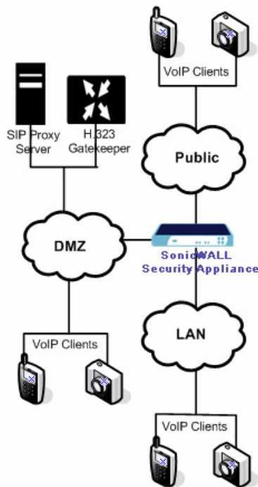
Figure 5 Trusted VoIP Service Topology.
