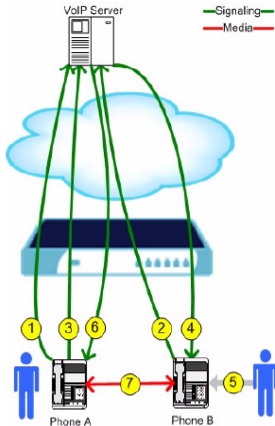
Figure 2 Local VoIP Call Flow
