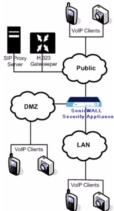
Figure 4 Public VoIP Service Topology.
