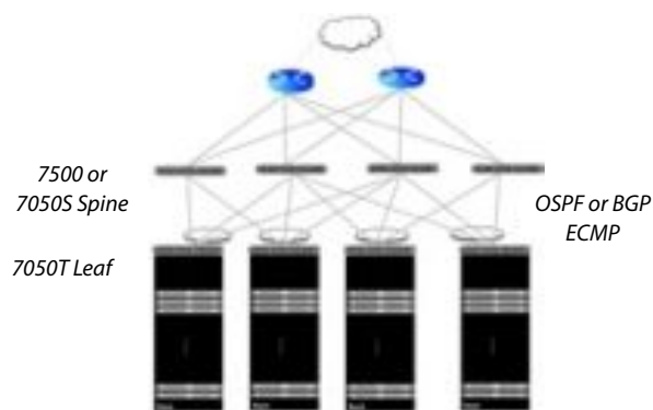
Arista Leaf-Spine Design with L3 ECMP
