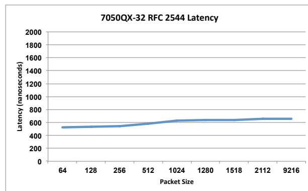
Arista 7050QX: Latency through QSFP+ ports
