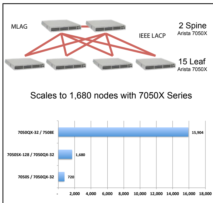
Arista Leaf-Spine Design with L2 MLAG
