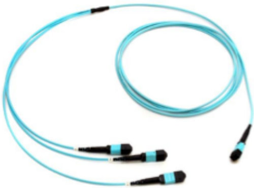
Figure 11: MTP-24 to 3 x MTP-12 Breakout Cable
