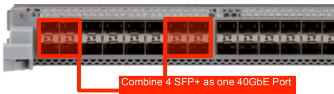
Figure 13: Agile Ports
