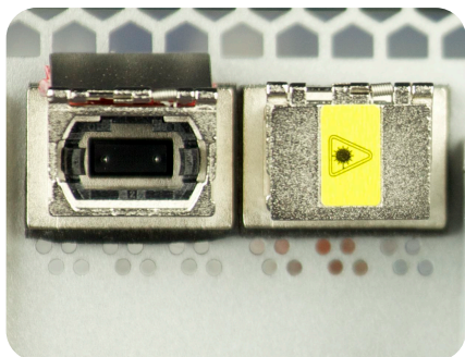
Figure 10: Arista MXP Interface for MTP-24 Cables
