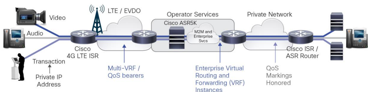
Figure 5. 4G LTE QoS
