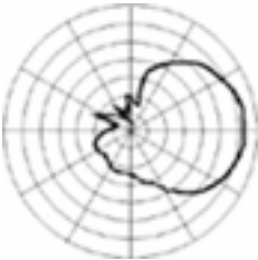
6dBi Patch Mode Vertical Radiation Pattern
