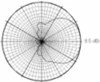
Vertical Radiation
