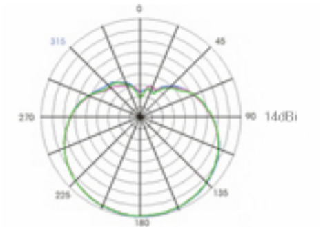
Vertical Radiation Pattern
