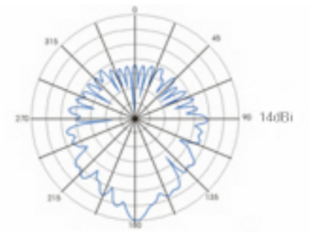
Horizontal Radiation Pattern
