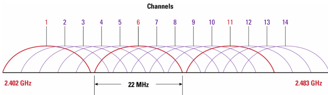
Figure 10. IEEE 802.11b DSSS Channel Allocations
