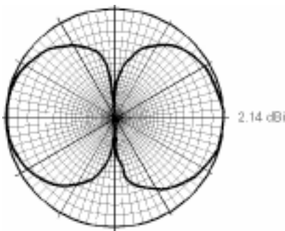
Vertical Radiation
