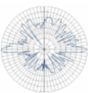
Radiation Pattern
