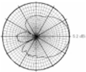
Vertical Radiation
