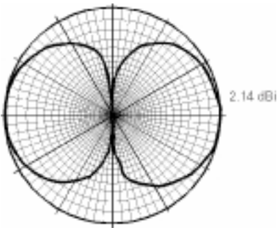
Vertical Radiation
