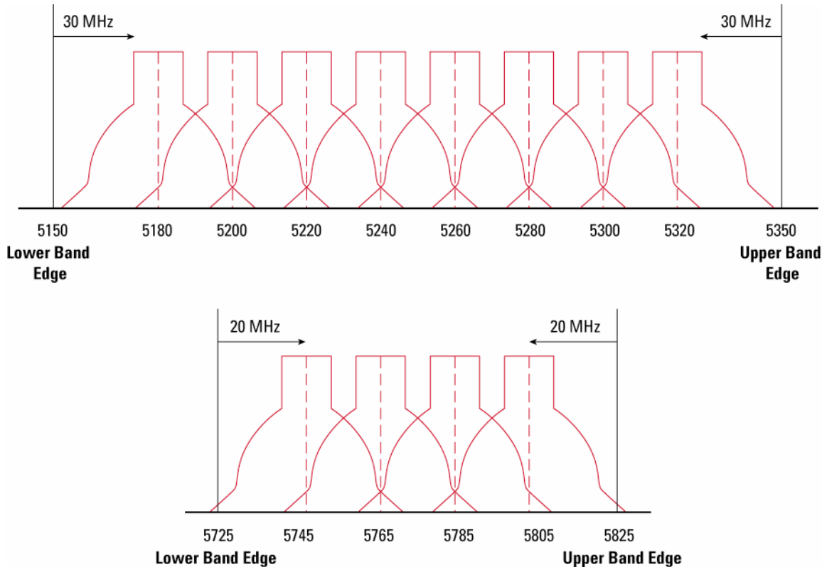
Figure 11. 802.11a Channel Allocation
