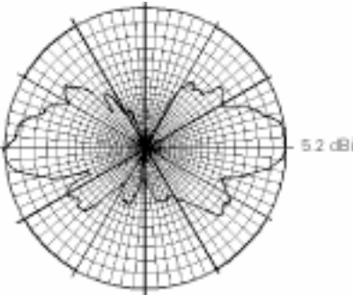
Vertical Radiation Pattern
