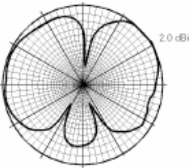
Vertical Radiation
