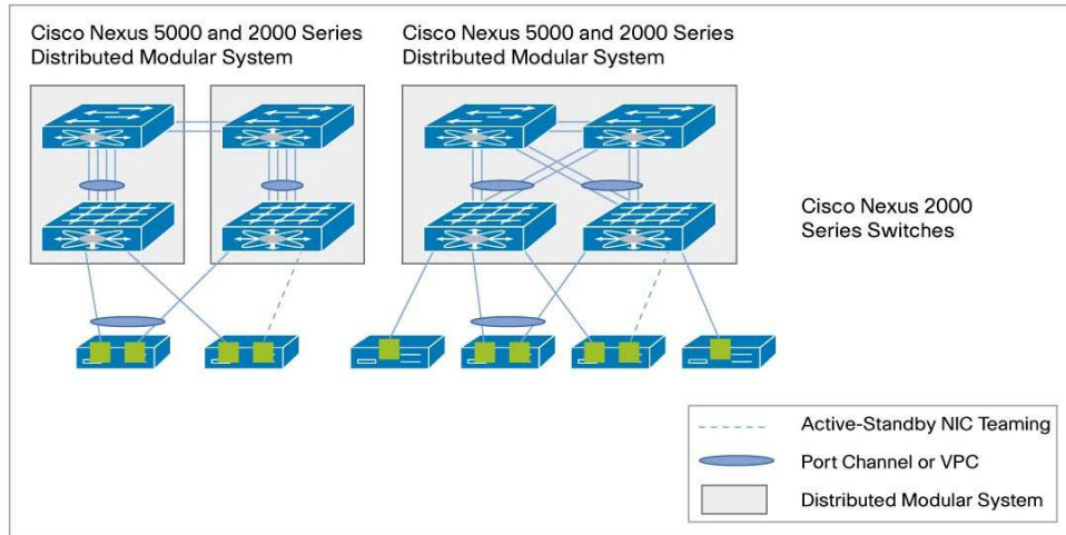
Figure 9. Deployment Scenario
