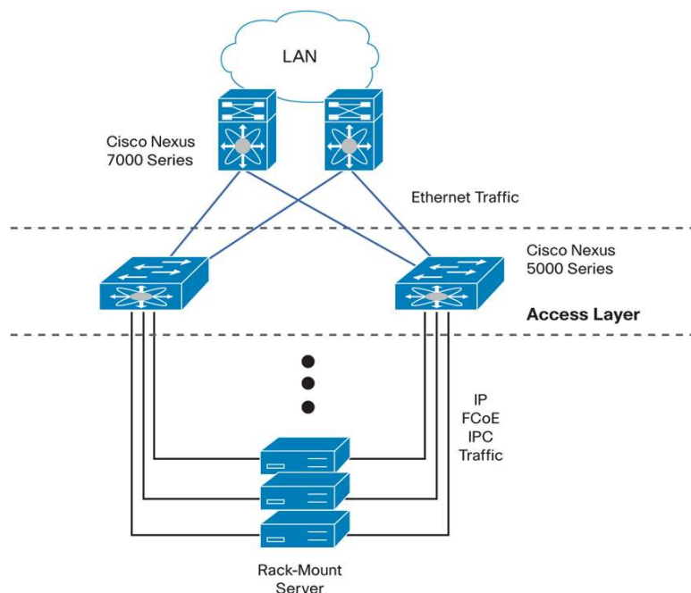
Figure 10. Active-Active Pair of Cisco Nexus 5000 Series Switches Connected to Redundant Servers
