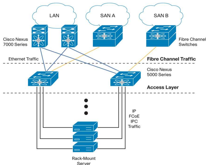
Figure 12. A Pair of Cisco Nexus 5000 Series Switches in an Active-Active Configuration with Native Fibre Channel Connections to Two Storage Networks
