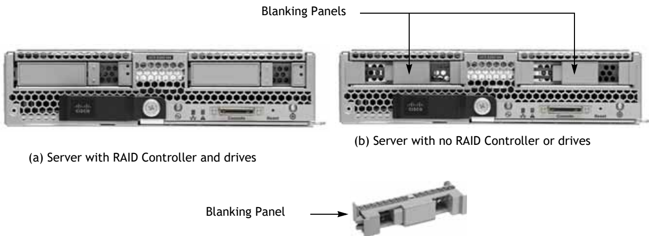
Figure 5 UCS B200 M4 With and Without RAID Controller (hidden) and Drives (Front View)
