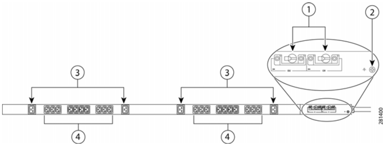
Figure 19 Zero Rack Unit PDU (PID = RP208-30-2P-U-2)
