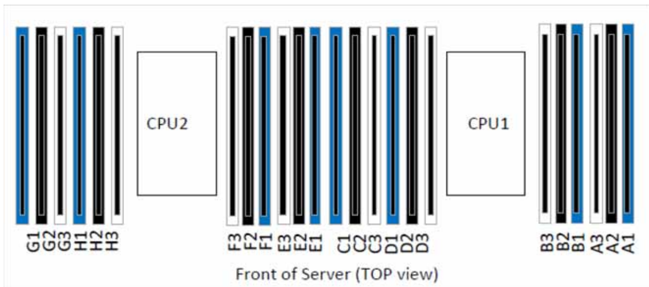
Figure 11 Physical Layout of CPU DIMM Channels and Slots
