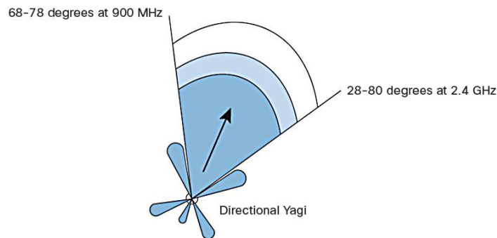
Figure 3. Yagi Antenna
