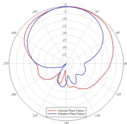
Azimuth and Elevation Radiation Patterns Right Antenna - 2.4 GHz Band
