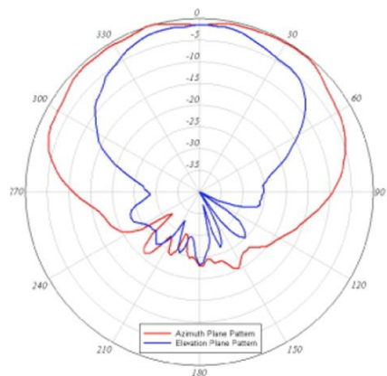
Azimuth and Elevation Radiation Patterns Right Antenna - 5 GHz Band
