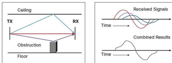
Figure 4. Multipath Distortion
