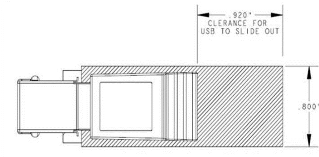
Figure 6 USB Clearance
