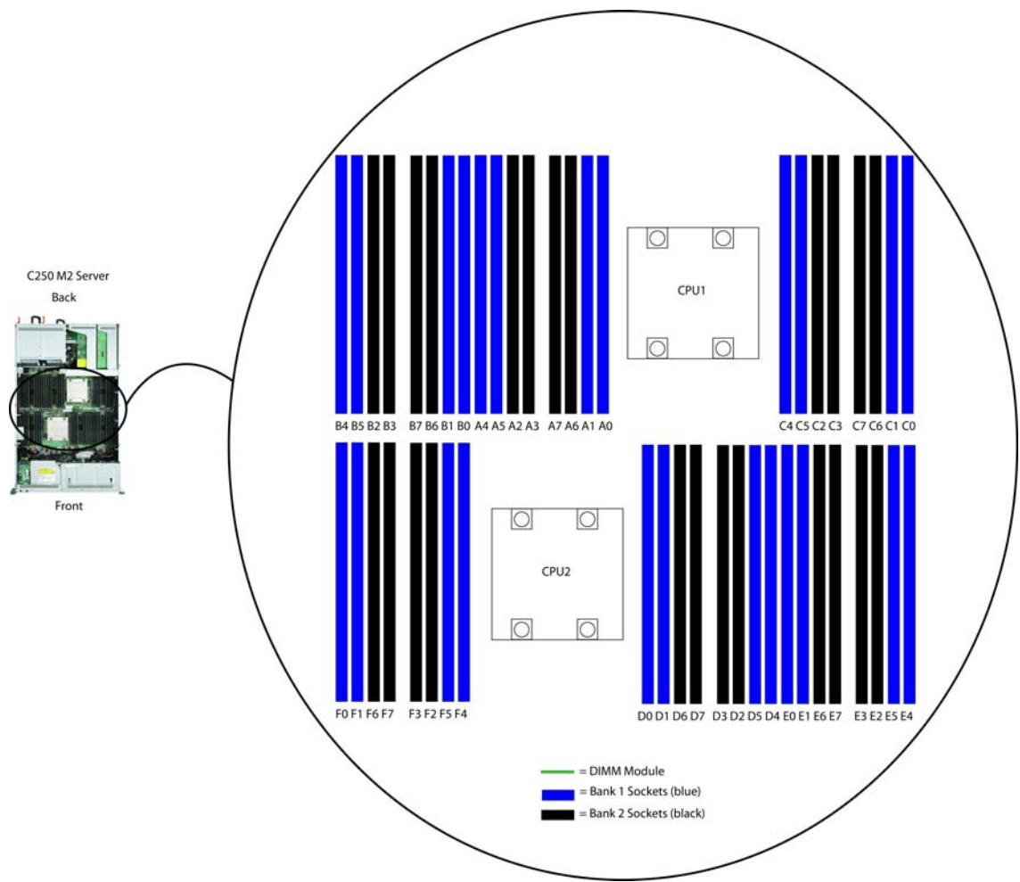
Figure 8 CPU DIMM Channels and Banks
