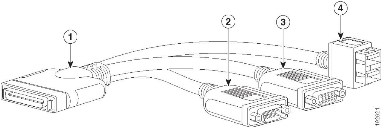
Figure 12 KVM Cable
