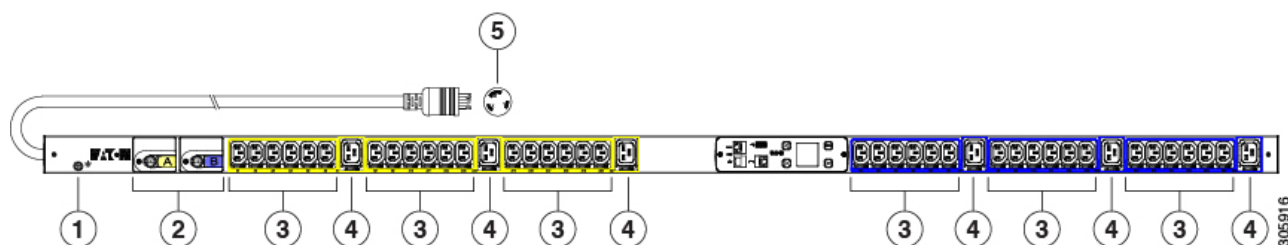
Figure 16 RP208-30M1P-6-36 PDU
