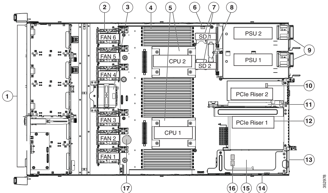
Figure 6 C220 M4 SFF With Top Cover Off
