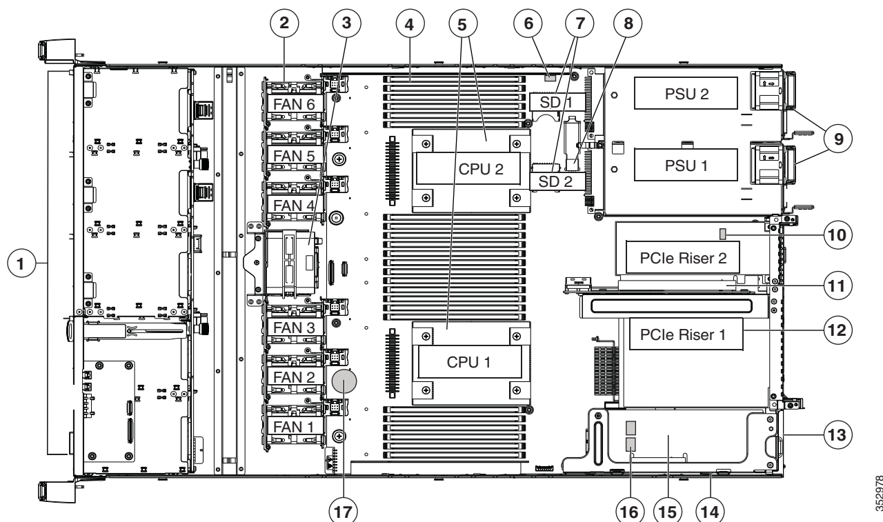
Figure 18 Motherboard USB and SD Ports and RAID Card SuperCap Location
