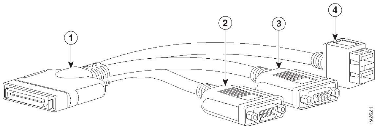
Figure 13 KVM Cable
