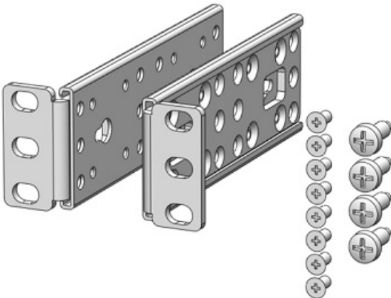
1U-N22-N32-FM-BR: N2200-ON/N3200-ON/E3200-ON Series/S3248T-ON MPS-1S flush-mount, offset-mount, or rear-mount brackets (PR8P0)
