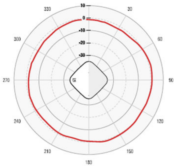
Azimuth - 5 GHz
