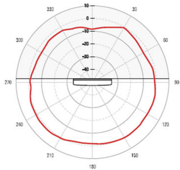
Elevation - 5 GHz
