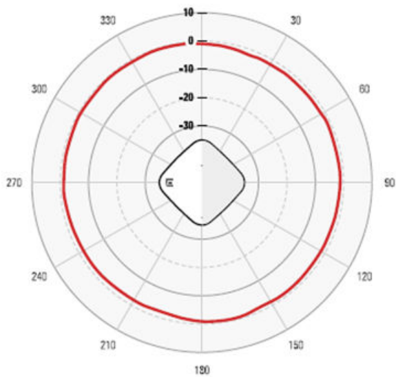
Azimuth - 5 GHz
