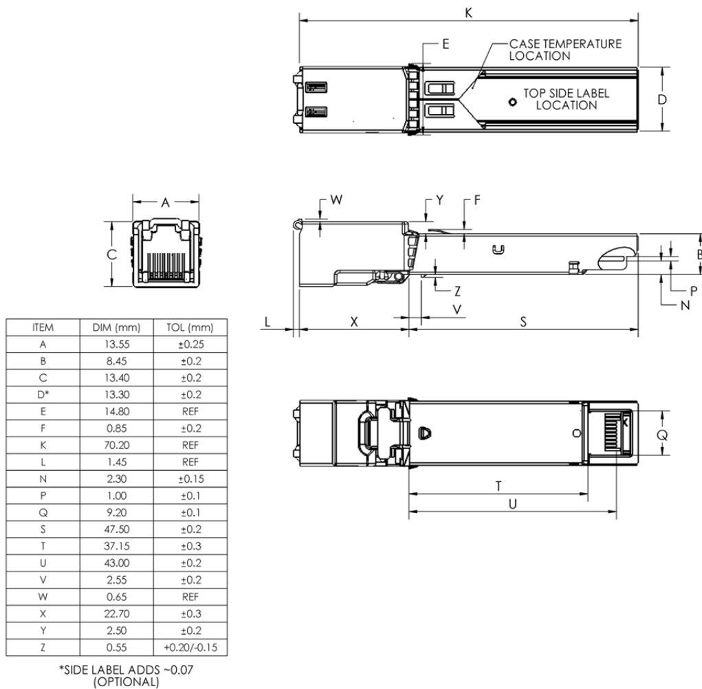
Figure 2. FCLF-8520/8521-3 mechanical dimensions
