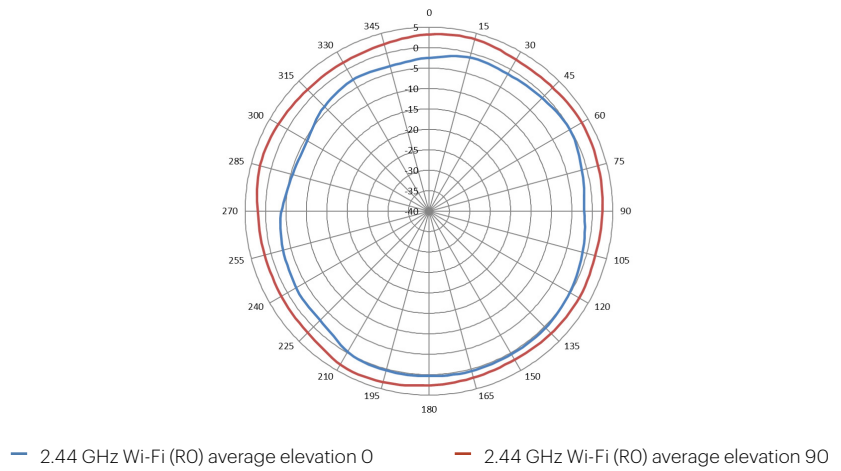
Figure 4. 2.44 GHz Wi-Fi antenna patterns (vertical)
