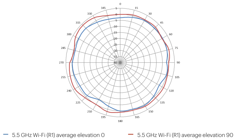
Figure 5. 5.5 GHz Wi-Fi antenna patterns (vertical)
