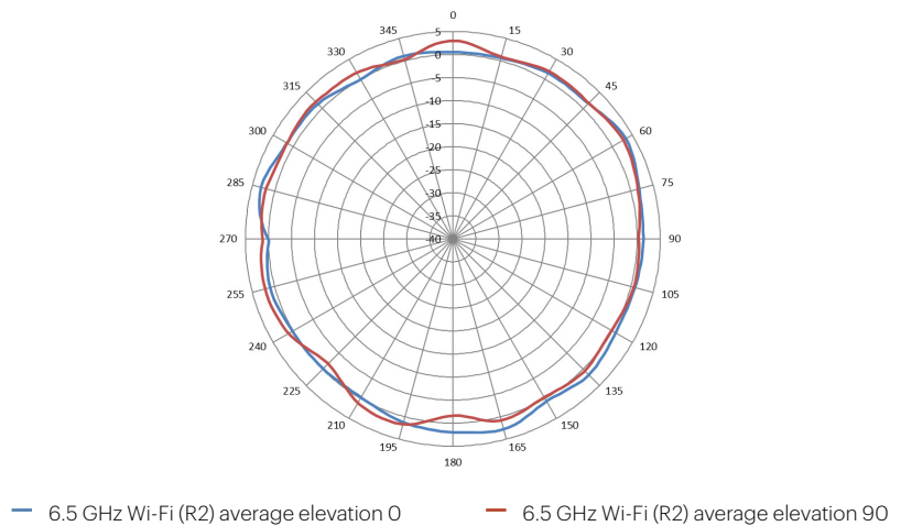
Figure 6. 6.5 GHz Wi-Fi antenna patterns (vertical)
