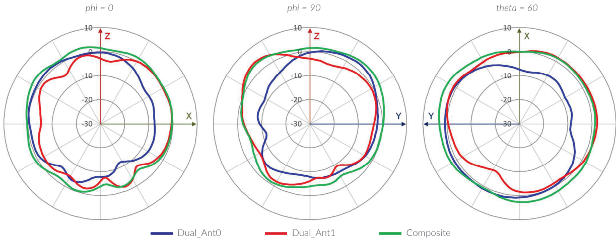
2.4 Ghz Wi-Fi @ 2400MHz (R1)
