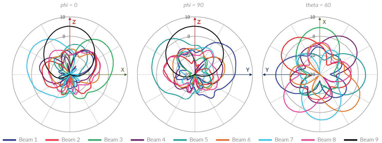
2.4 Ghz Directional BLE @ 2400MHz
