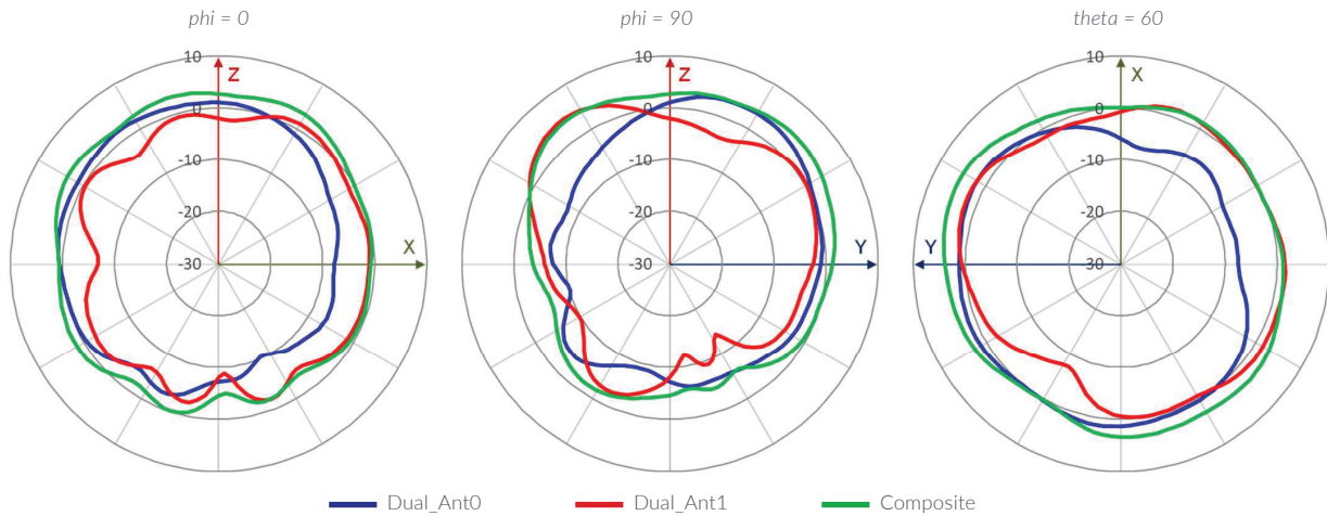
2.4 Ghz Wi-Fi @ 2450MHz (R1)
