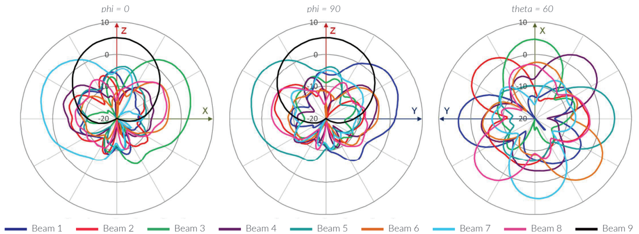
2.4 Ghz Directional BLE @ 2440MHz
