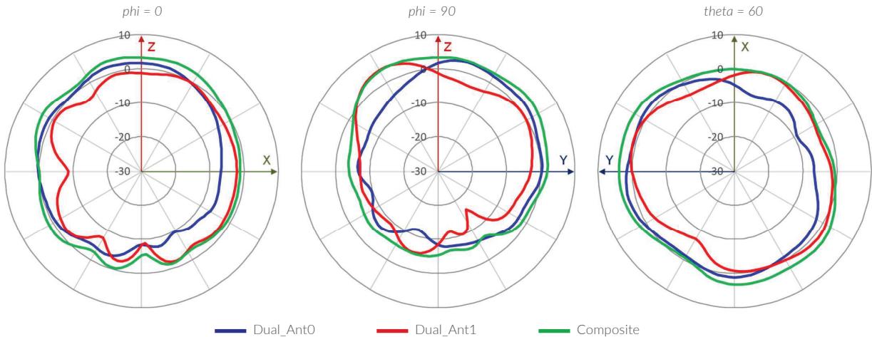
2.4 Ghz Wi-Fi @ 2500MHz (R1)
