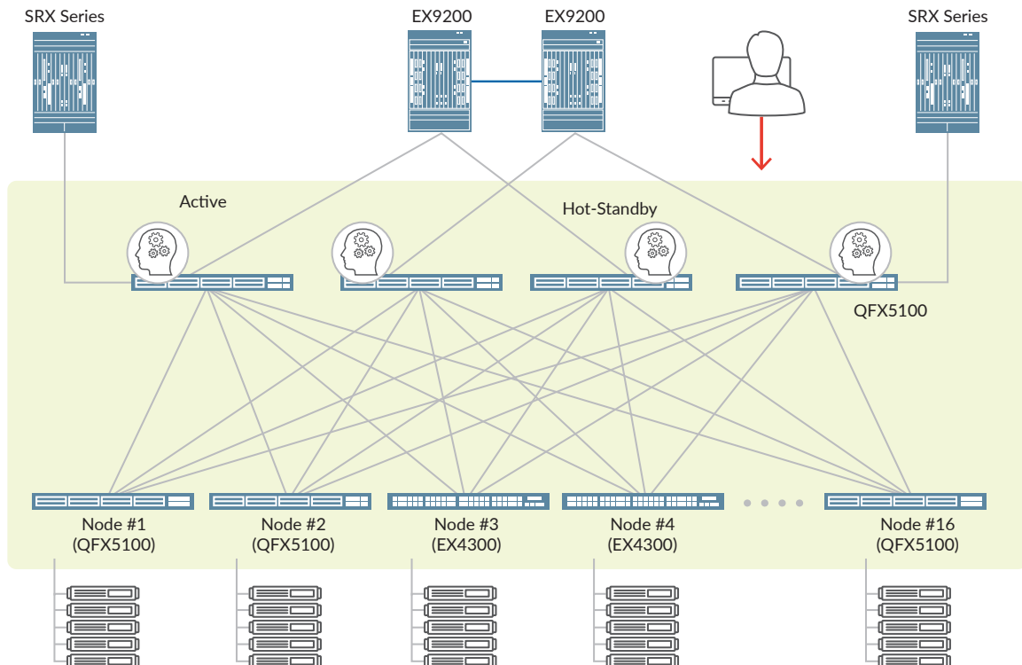
Figure 5: Virtual Chassis Fabric data center deployment with a mix of 1GbE and 10GbE
