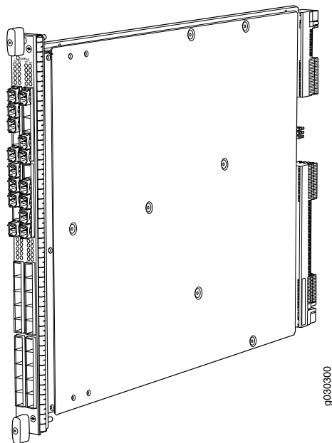
Figure 7: IOC SRX5K-40GE-SFP
