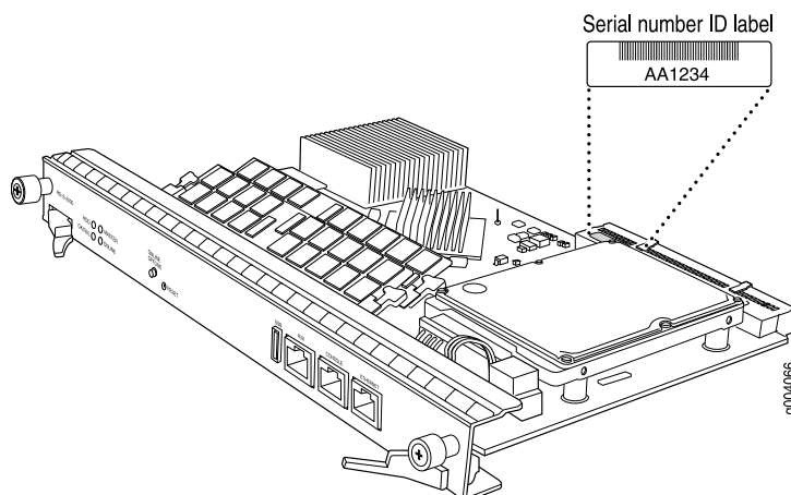
Figure 44: SRX5K-RE-13-20 Serial Number Label
