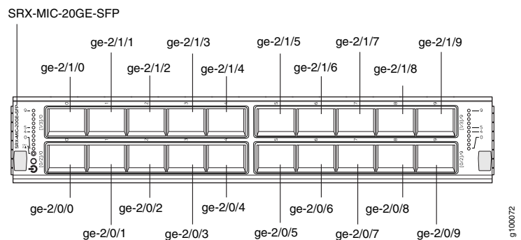
Figure 13: SRX-MIC-20GE-SFP Interface Port Mapping
