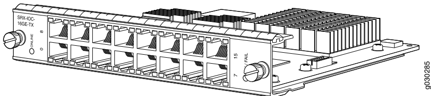
Figure 34: Flex IOC Port Module SRX-IOC-16GE-TX
