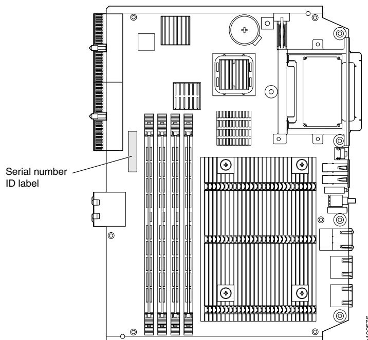
Figure 47: SRX5K-RE3-128G Serial Number Label
