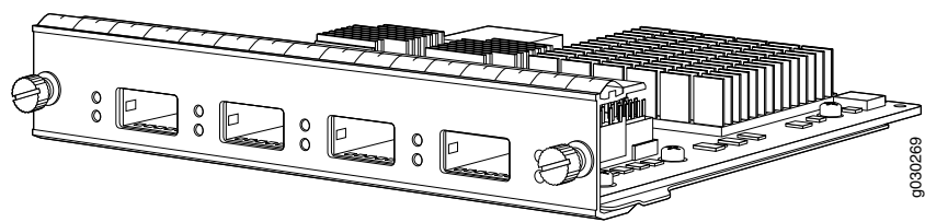
Figure 36: Flex IOC Port Module SRX-IOC-4XGE-XFP
