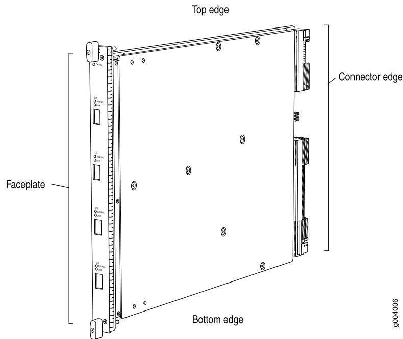
Figure 48: Card Edges
