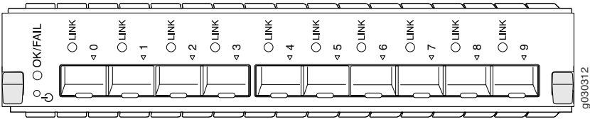
Figure 15: SRX-MIC-10XG SFPP
