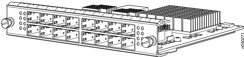
Figure 32: Flex IOC Port Module SRX-IOC-16GE-SFP
