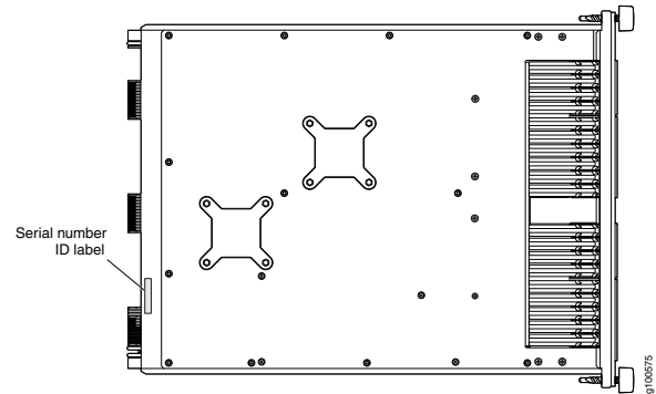
Figure 27: SRX5K-IOC4-10G Serial Number Label
