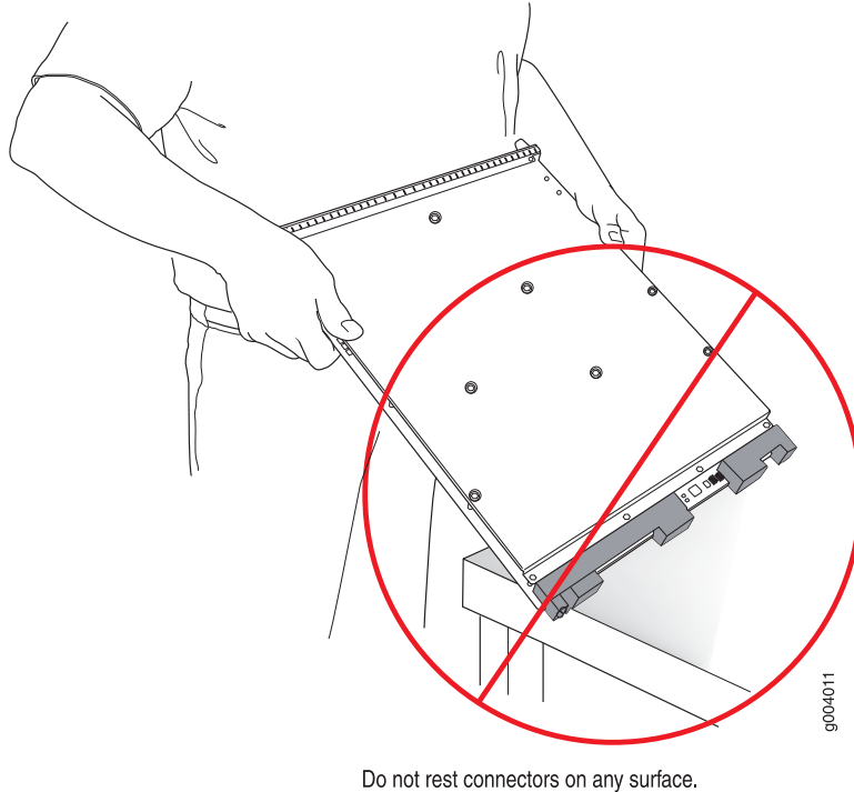
Figure 50: Do Not Rest the Card on an Edge
