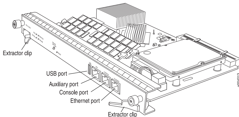
Figure 43: Routing Engine
