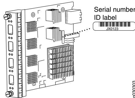
Figure 37: Port Module SRX-IOC-4XGE-XFP Serial Number Label
