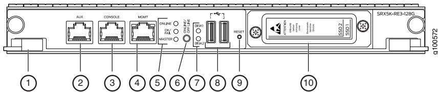
Figure 46: SRX5K-RE3-128G Routing Engine Front View
