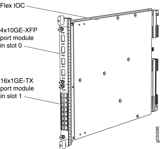
Figure 30: Flex IOC with Typical Port Modules
