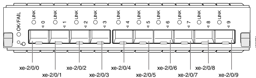
Figure 16: SRX-MIC-10XG-SFPP Port and Interface Numbering
