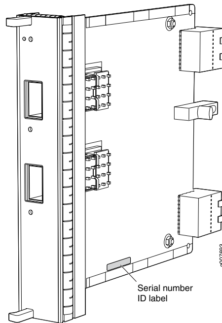
Figure 21: SRX-MIC-2X40G-QSFP Serial Number Label
