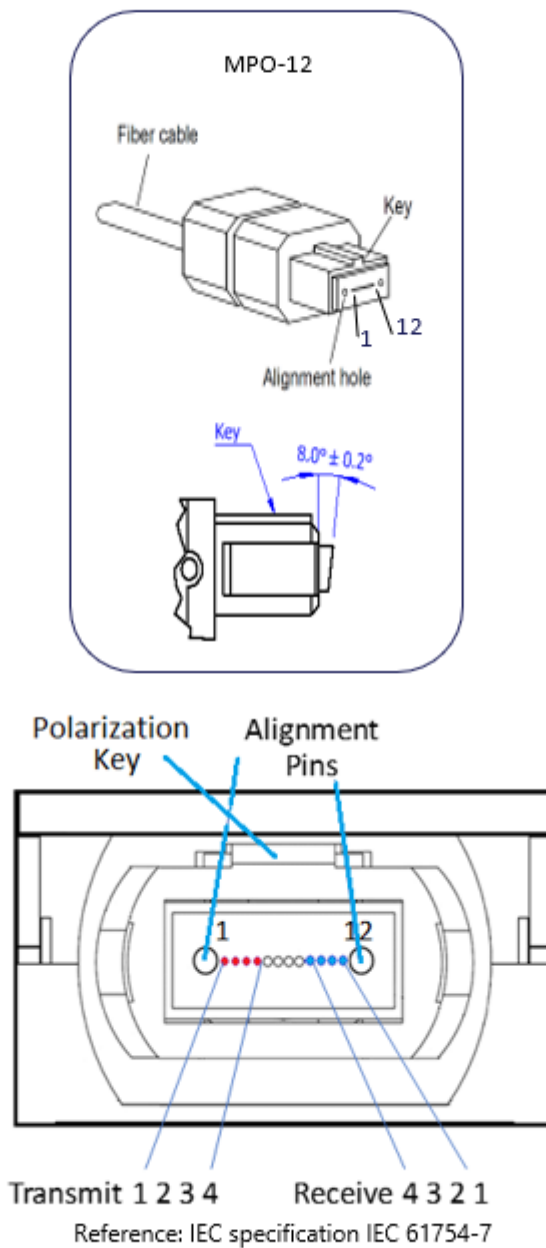
NDR transceiver: MPO Receptacle, Lane Assignment, and Positioning Key (front view)
