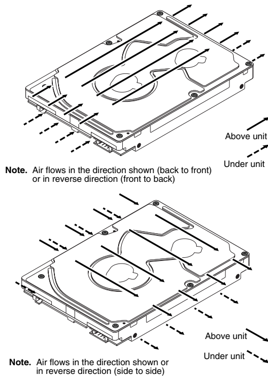
Figure 9. Air flow
